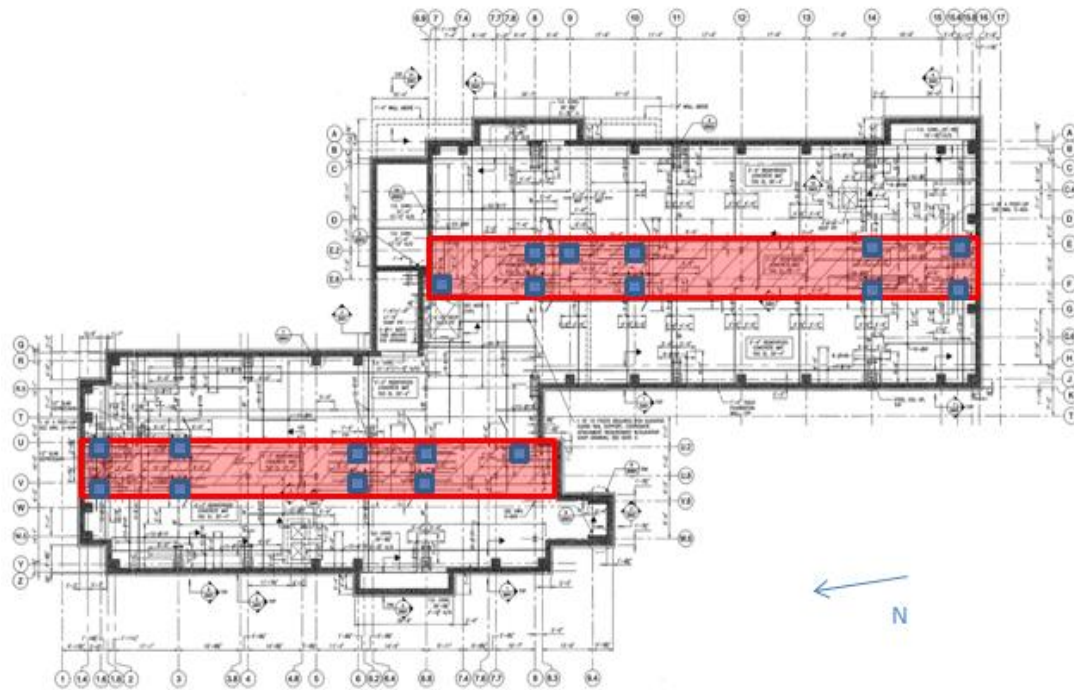
Figure 2: Foundation Trench
